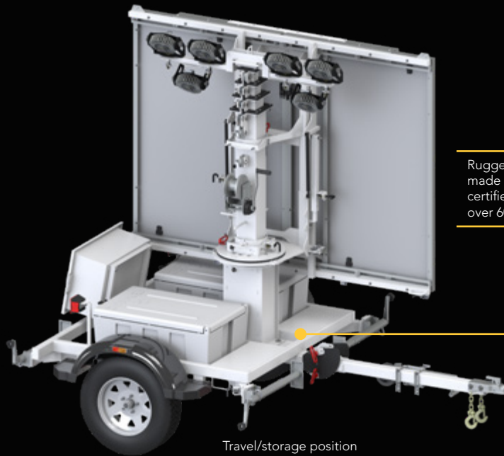
Travel/storage position
